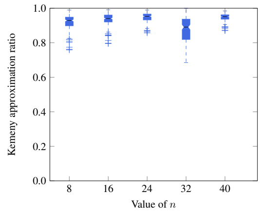
(a) NAIVE-BIPARTITE
